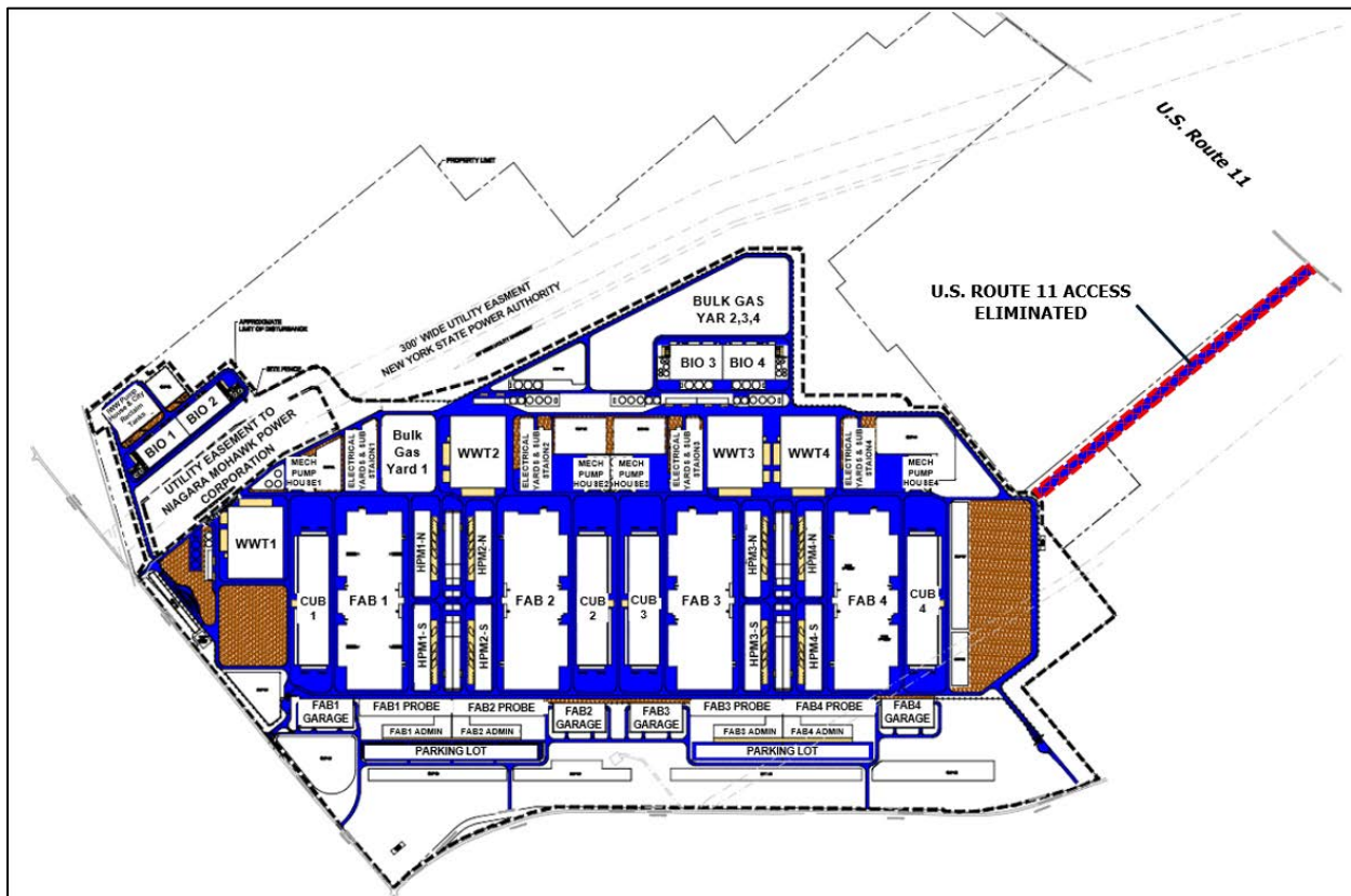
Figure 2.2-2 U.S. Route 11 Access Elimination Layout
