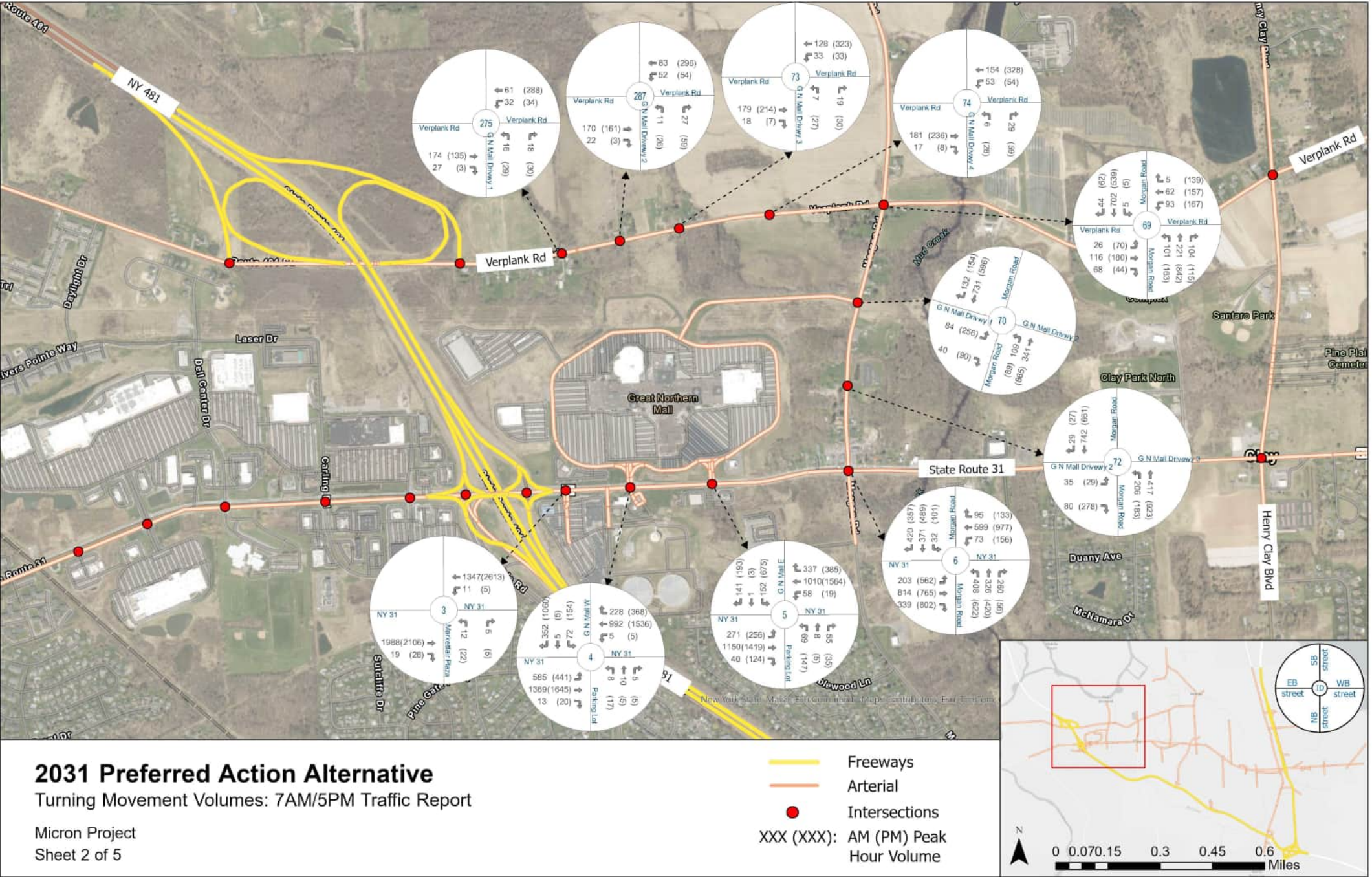
Figure 8-11: Year 2031 Preferred Action Alternative 7AM/5PM Traffic Volumes - Intersections - Sheet 2 of 5
