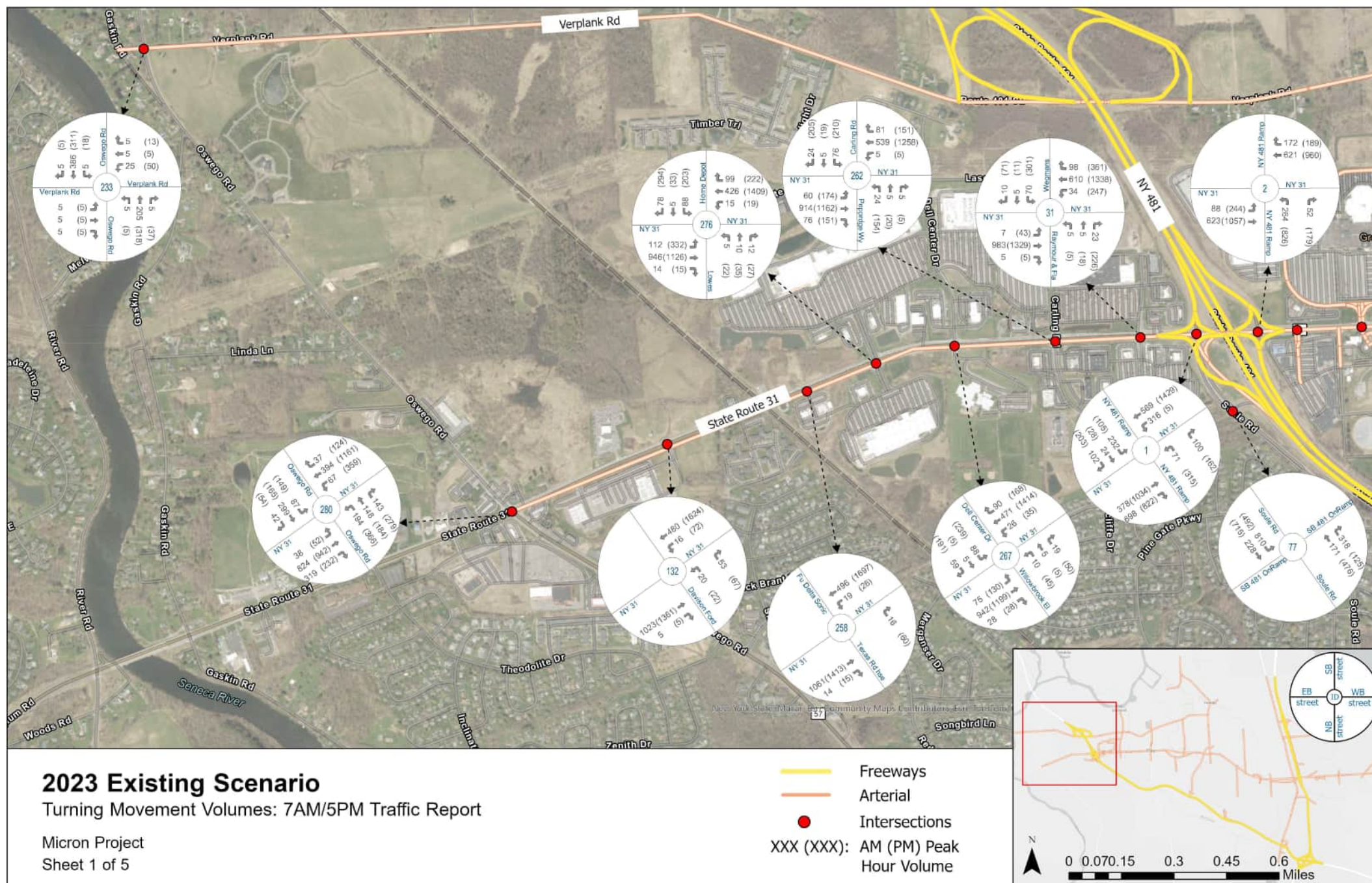
Figure 5-3: Year 2023 Existing 7AM/5PM Peak Hour Traffic Volumes - Intersections - Sheet 1 of 5
