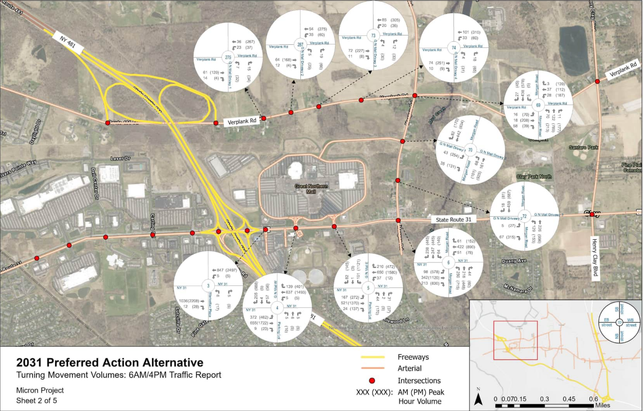
Figure 8-9: Year 2031 Preferred Action Alternative 6AM/4PM Traffic Volumes - Intersections - Sheet 2 of 5
