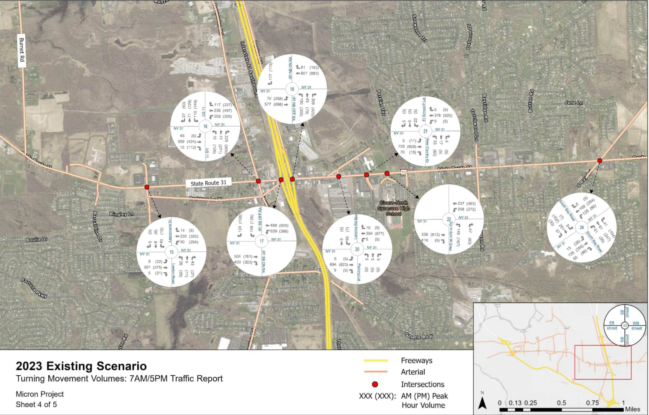
Figure 5-3: Year 2023 Existing 7AM/5PM Peak Hour Traffic Volumes - Intersections - Sheet 4 of 5
