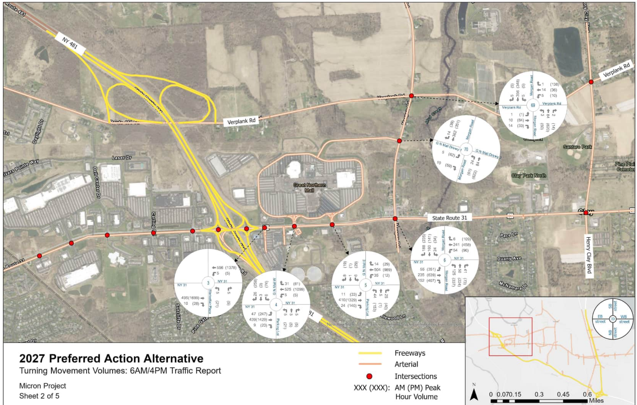
Figure 7-9: Year 2027 Preferred Action Alternative 6AM/4PM Traffic Volumes - Intersections - Sheet 2 of 5
