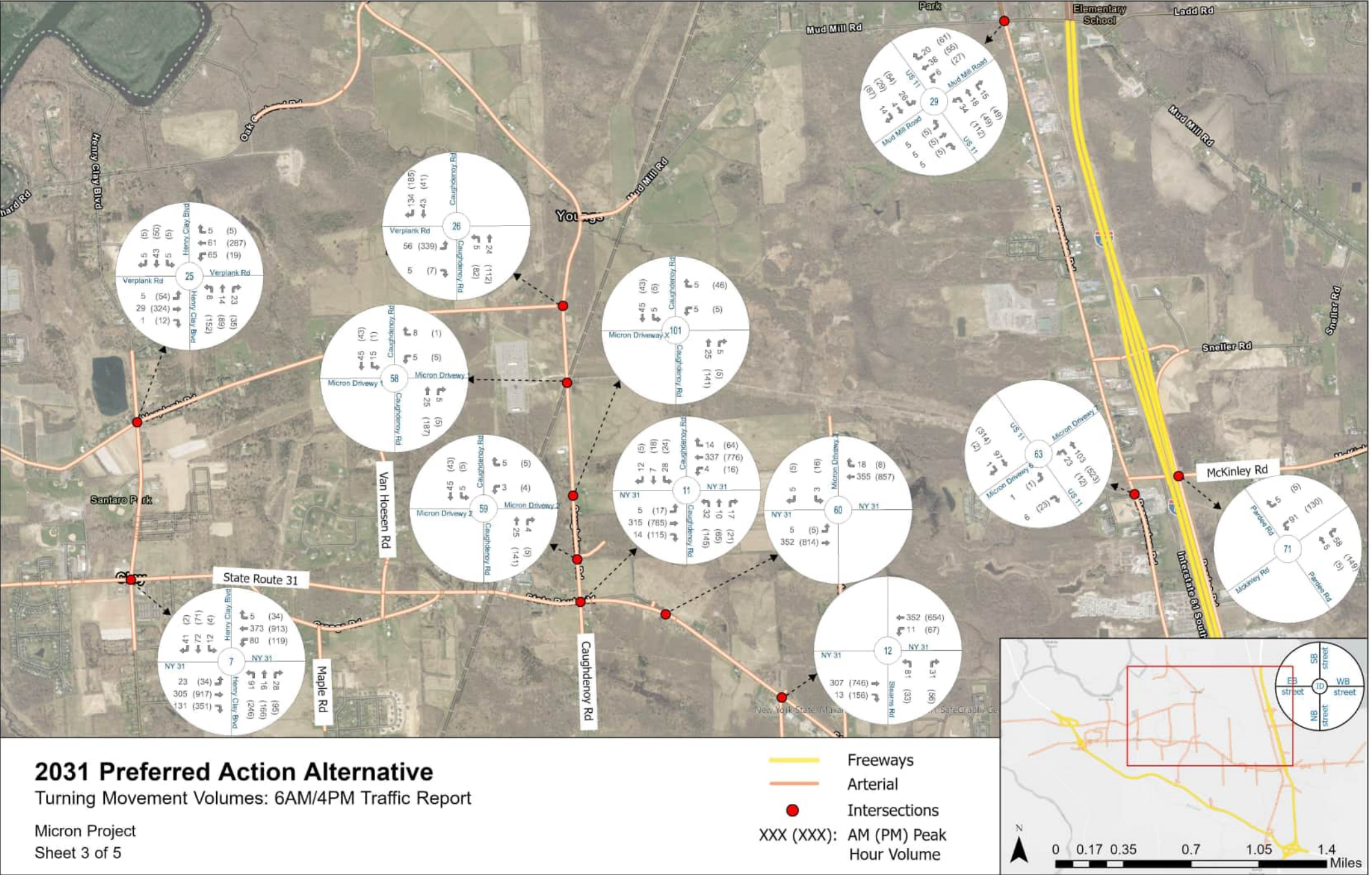
Figure 8-9: Year 2031 Preferred Action Alternative 6AM/4PM Traffic Volumes - Intersections - Sheet 3 of 5
