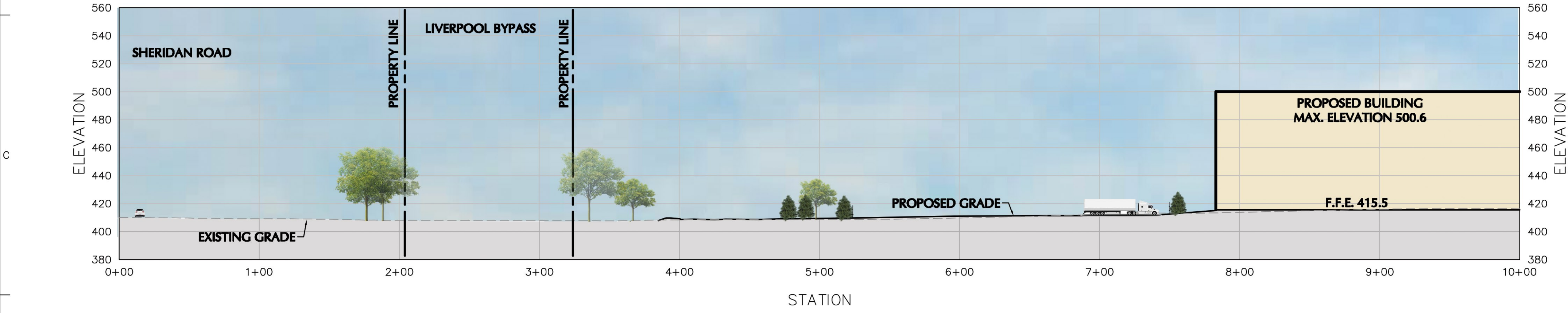
SECTION B-B' (1) PROFILE
