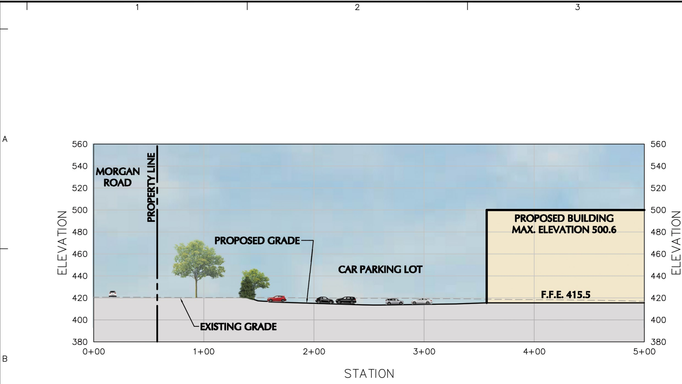
SECTION A-A' (1) PROFILE
