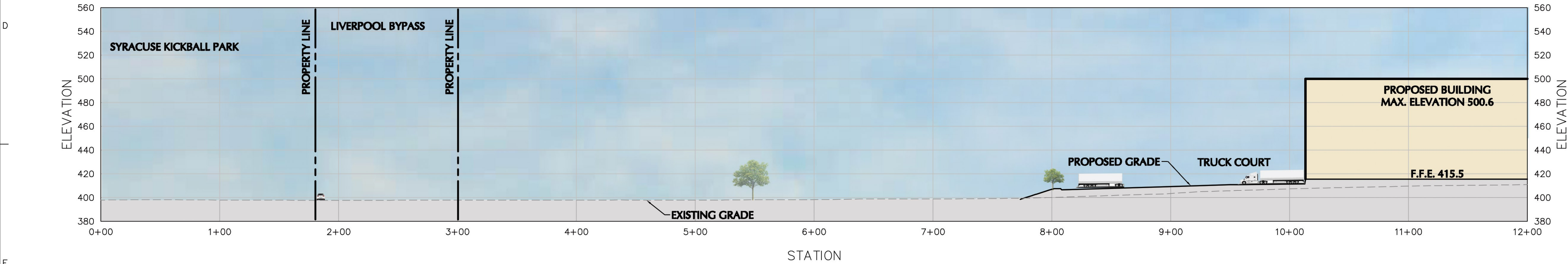
SECTION C-C' (1) PROFILE
